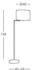
1264.41.6 Bodenleuchte / floor lamp vernickelt / nickel plated 1 Ip., E27, 60 W / LED E27
