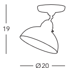
731.10.100 Deckenleuchte/ ceiling lamp 1 Ip., E27, 75 W/ LED E27
